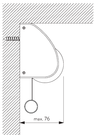
Direct fitting
