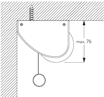
Direct fitting
