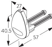
SG 4944 Side guide end cover
