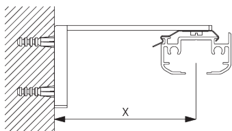
Smart Fix SG 11201 - SG 11204 and bracket SG 2616: Screw SG 10395 (M4x6) needed
